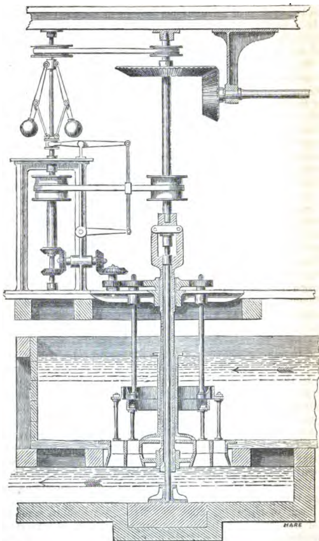
Fig. 14.—Sectional Elevation.
